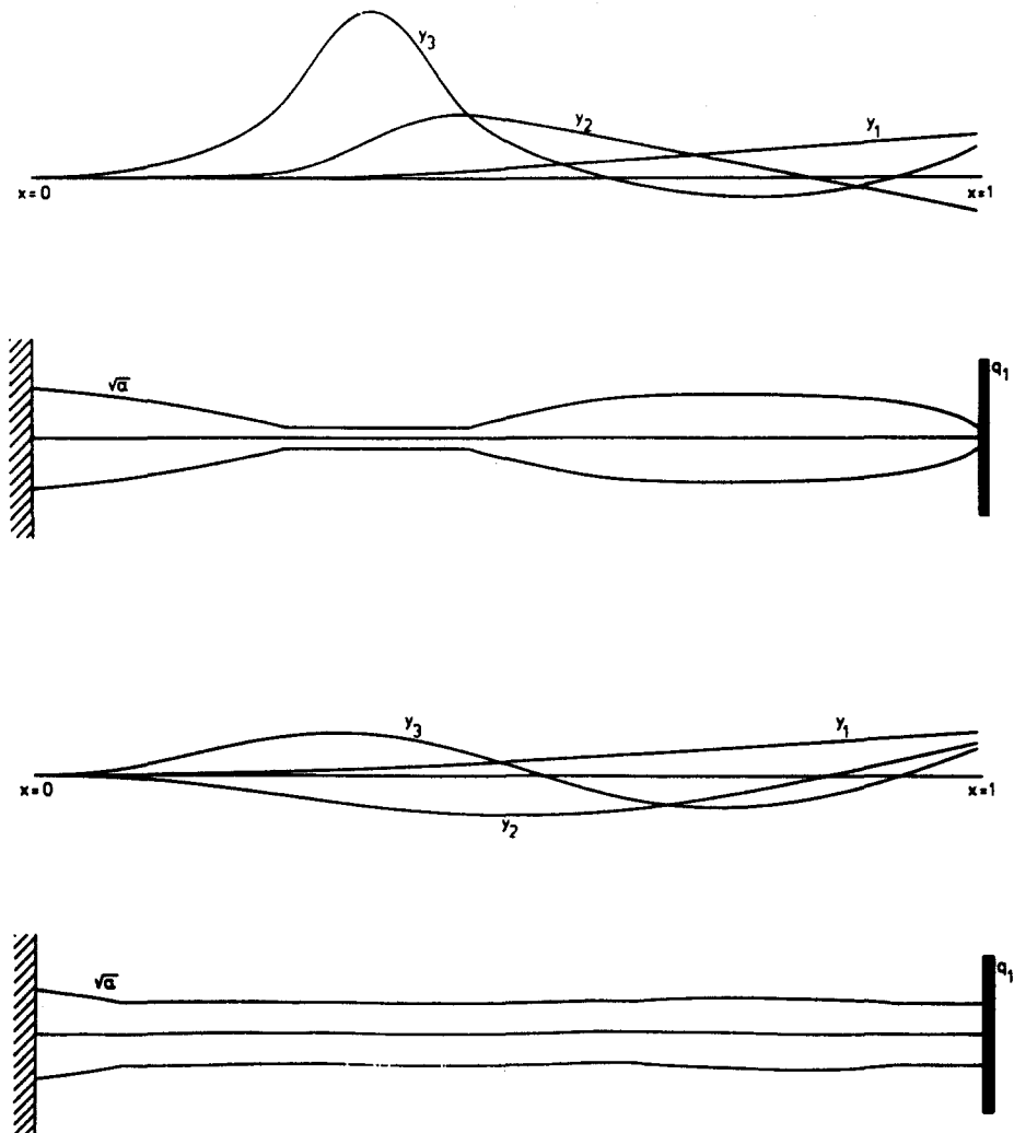
Fig. 3. Optimal \omega_3 - \omega_2 cantilevers with tip mass q_1 = Q_1/\rho V = 0.1 . The solution above has \bar{\alpha} = \bar{A}L/V = 0.1 , and has \omega_3 = \Omega_3(\rho L^3/cEV)^{1/2} = 92.4 , \omega_2 = 10.4 , and (\omega_3 - \omega_2)/(\omega_3^* - \omega_2^*) = \Delta\omega/\Delta\omega^* = 2.27 . The solution below has \bar{\alpha} = 0.9 , \omega_3 = 60.0 , \omega_2 = 20.4 , \Delta\omega/\Delta\omega^* = 1.09 .
