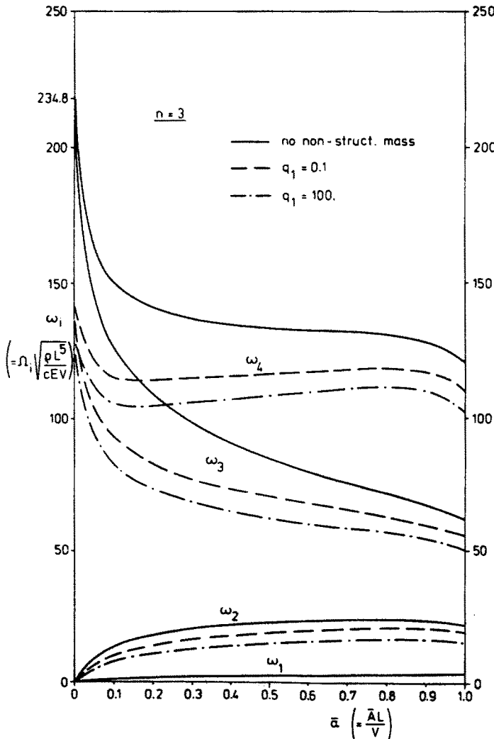
Fig. 1. Eigenfrequencies of optimal \omega_1 - \omega_2 cantilevers vs. minimum cross-sectional area constraint \bar{\alpha} .
